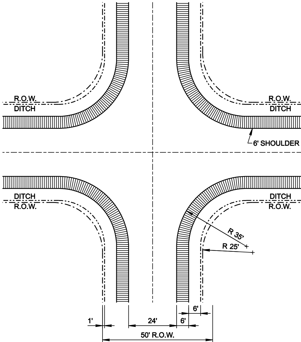
MINIMUM STANDARD PLAN FOR COLLECTOR STREETS (DITCH SECTION SHOWN) (NOT TO SCALE)
